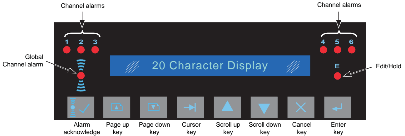
Figure 2.4 Operator interface
