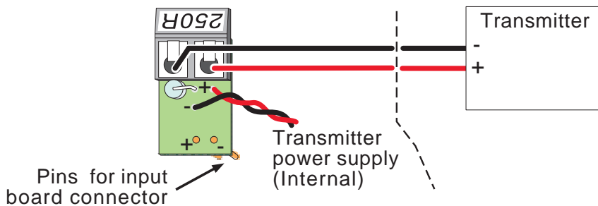
Figure 13.2b Transmitter wiring (internal power supply)
