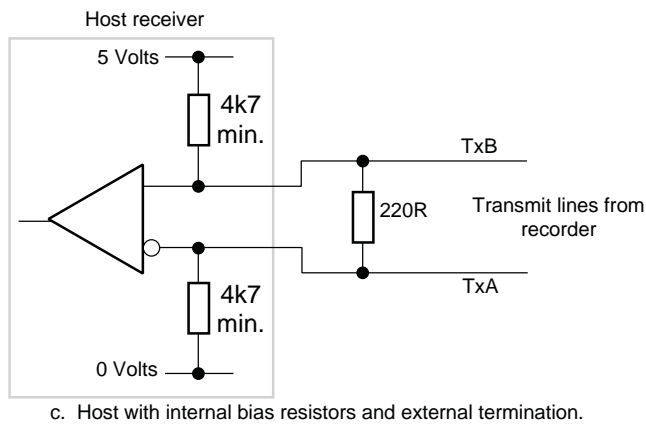
Figure 11.2.2b Host computer termination and biasing
