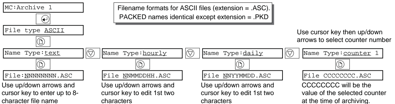
Figure 12.7 Filename selection
