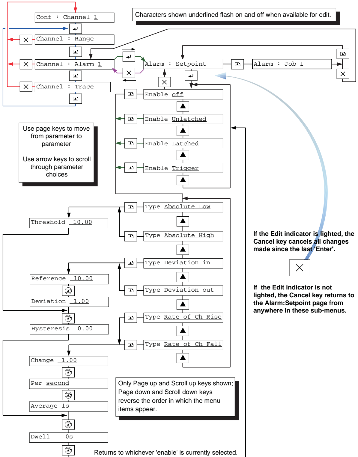
Figure 4.2 Configuration techniques
