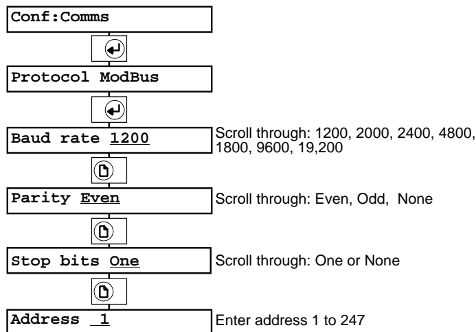
Figure 11.3 Configuration pages
