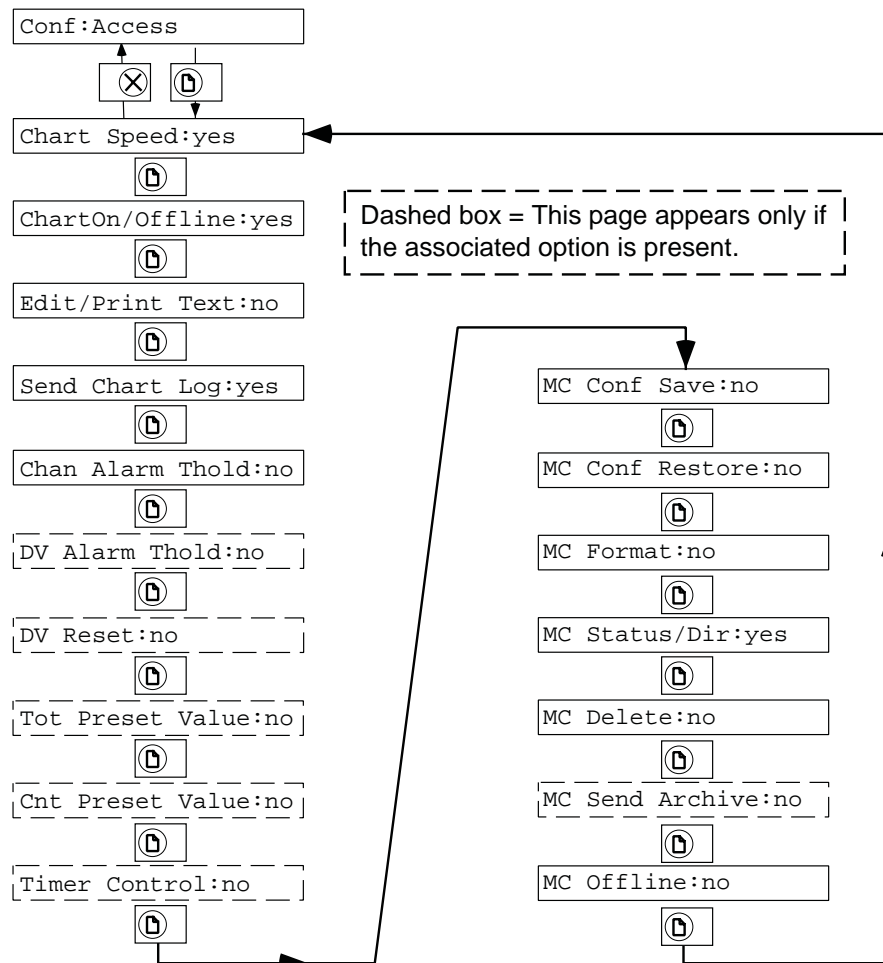
Figure 12.5 Operator permissions
